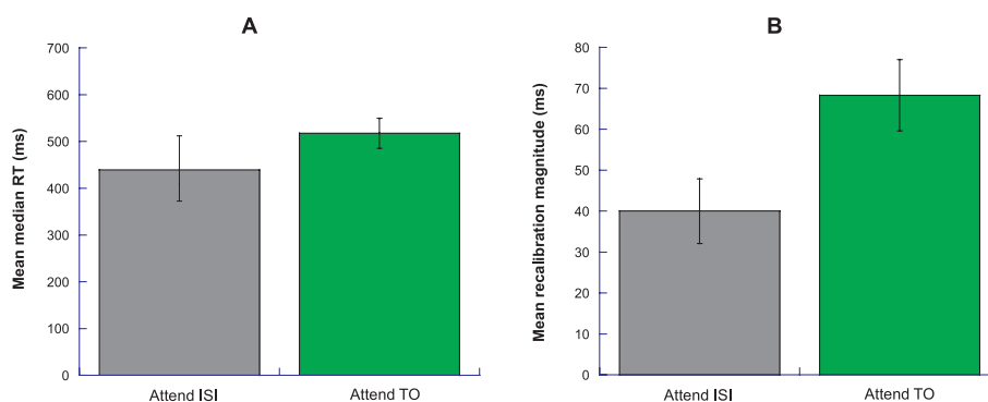
FIG. 5. Attending to ISI vs. attending to temporal order. (A) Grey bar represents mean median RT data for a condition in which observers attended to the ISI separating audiovisual stimulus pairs (as opposed to the within-pair audiovisual asynchrony) by detecting the presence of oddball ISI that were 400 ms shorter than the standard ISI length from the same experiment. The green bar represents 'attend temporal order' RT data taken from Fig. 3B. (B) Grey bar represents mean recalibration magnitude ( n = 4 ) from the same experiment. The green bar represents the 'attend temporal order' recalibration data taken from Fig. 2B.
