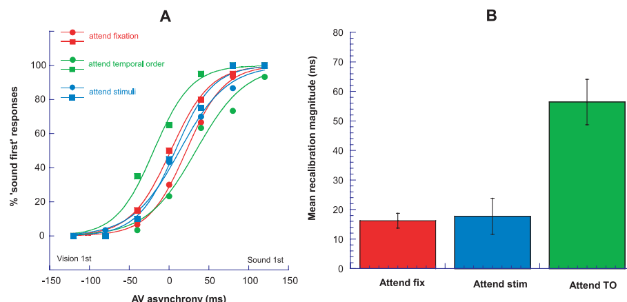
FIG. 2. Attentional modulation of temporal adaptation. (A) Sample psychometric functions from one representative observer showing temporal-order judgments (TOJs) as a function of audiovisual (AV) asynchrony. Square and circle data points represent TOJs following adaptation to 120 ms visual or auditory temporal leads, respectively. Different colours represent conditions in which observers were presented with physically identical stimuli but shifted the focus of their selective attention toward either a fixation cross (red), nontemporal features of the adapting stimuli (blue) or the temporal order of the adapting stimuli (green). For each function, the point of subjective simultaneity (PSS) represents the physical asynchrony value corresponding to perceptual simultaneity (50% 'sound first' responses). (B) Recalibration magnitude averaged across observers ( n = 7 ) for each attention condition (fix, fixation cross; stim, stimuli; TO, temporal order). The height of the bars represents the arithmetic difference between PSS values from functions of the same colour shown in A (i.e. opposing adaption asynchrony polarities). The same colour coding applies to both A and B. Error bars represent the SEM between observers.
